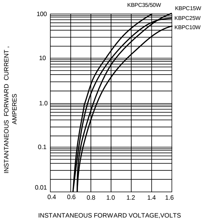
FIG.3-TYPICAL FORWARD CHARACTERISTICS
