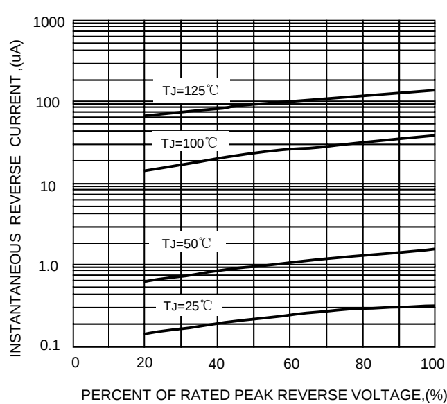
FIG.3-TYPICAL REVERSE CHARACTERISTICS
