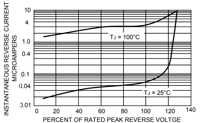
FIG.6-TYPICAL REVERSE CHARACTERISTICS
