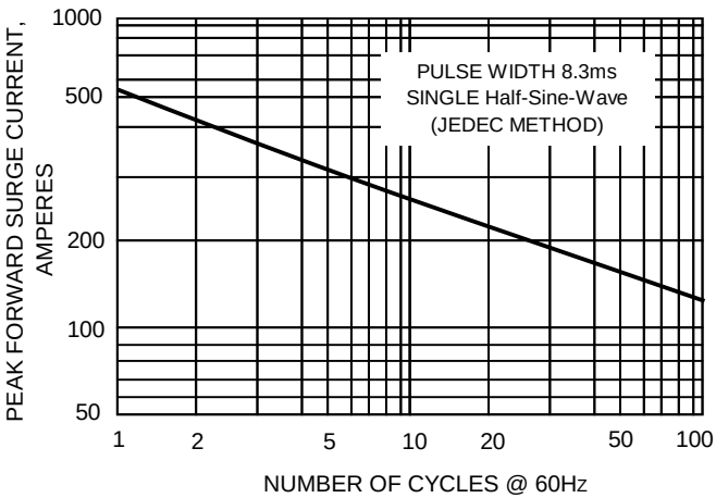
FIG.2- NON-REPETITIVE PEAK FORWARD SURGE CURRENT
