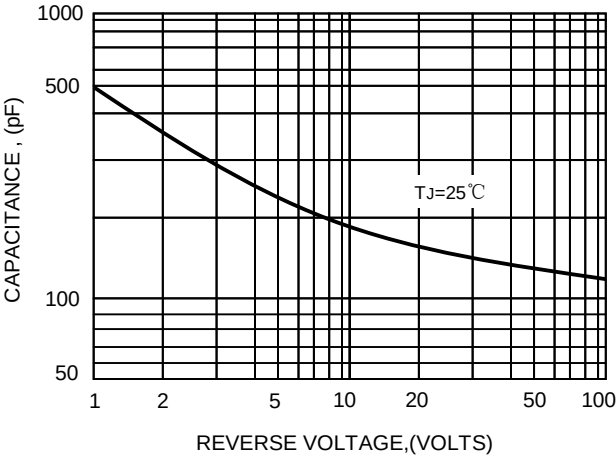
FIG.5-TYPICAL JUNCTION CAPACITANCE
